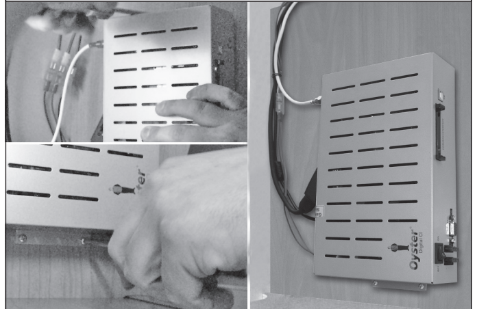
4. Optional: Wandmontage / mounting on wall / montage mural
